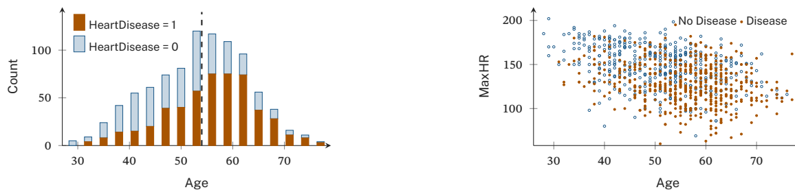
Figure 1. Exploratory views of all 918 patients. Three-year age bins start at 27.5; the dashed line marks the median age of 54. The scatter usesunjittered observations, so coincident points overlap. Neither plot fits a model.
